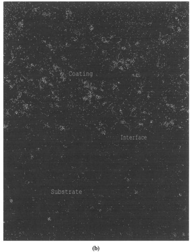
Fig. 10 (a) Al-50SiC22 coating on an Al foil showing absence of a regular interface. (b) Si map of (a) showing the distribution of the SiC. (Art has been reduced to 43% of its original size for printing.)
