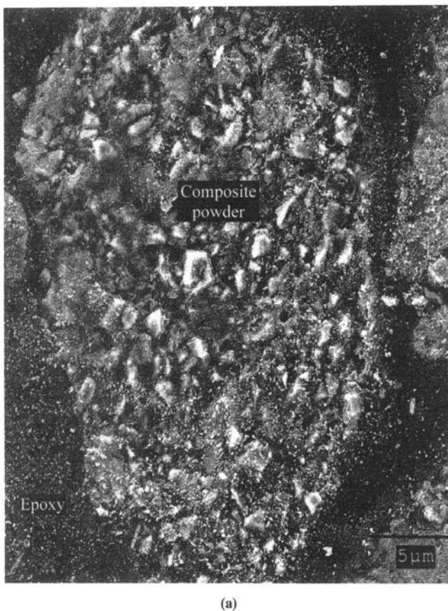
Fig. 1 (a) Cross section of an Al-50SiC8 powder milled for 1800 s with process control agent (PCA) as an additive. (Art has been reduced to 43% of its original size for printing.) (b) Cross section of an Al-50SiC8 powder milled for 1800 s without PCA. (Art has been reduced to 42% of its original size for printing.)
