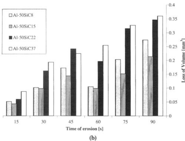
Fig. 13 (a) Variation of erosive wear resistance with SiC content in the Al-SiC composites containing 8 \mu\text{m} large SiC. (Data for the wear of the reference cast composite material was not available for t = 60 s.) and (b) change in erosion wear resistance with SiC particle sizes for the Al-SiC composites containing 50 vol% SiC
