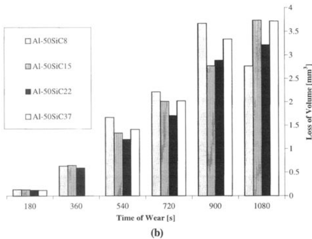
Fig. 11 Change in abrasive wear resistance with SiC content under a load of 35 N for the Al-SiC composites containing (a) 8 \mu\text{m} large SiC and (b) 50 vol% SiC
