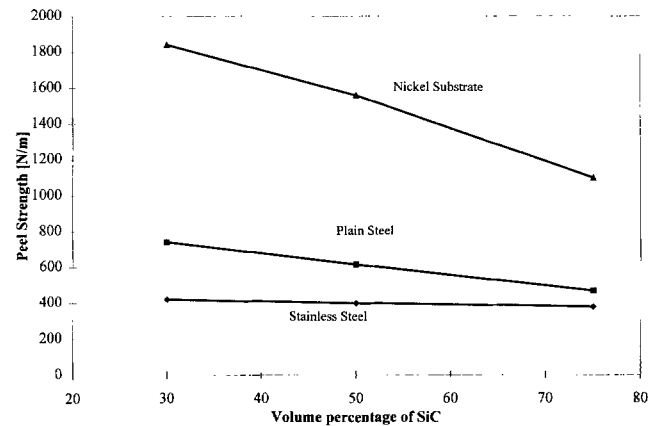
Fig. 8 Variation of the average peel strength with SiC content for different substrates
